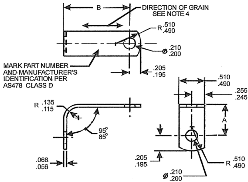
FIGURE 1 - ANGLE BRACKET
